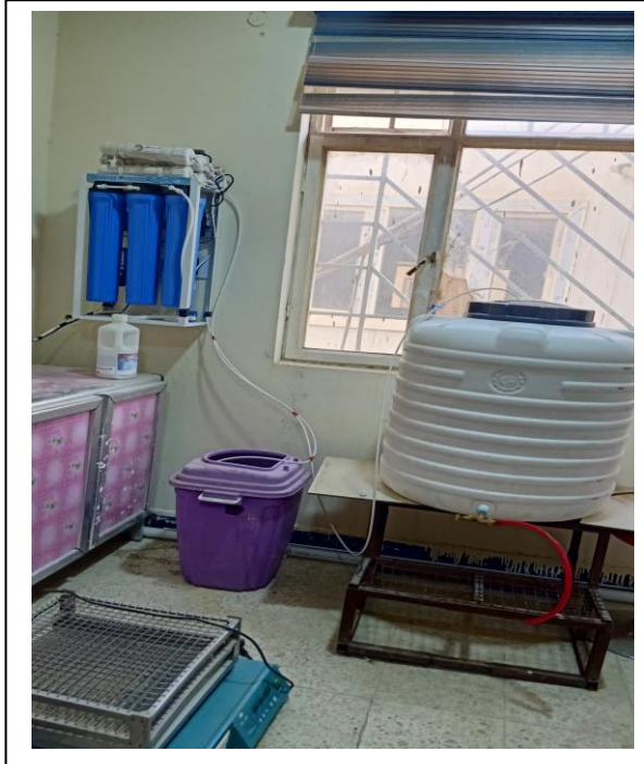
RO system to treat drinking water, College of agriculture
